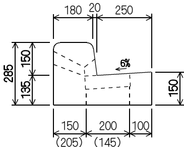
縁塊 (94kg)
